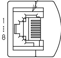
MJ1 (8極 8心RJ48)
