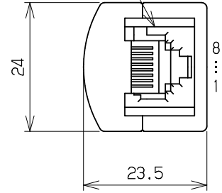
MJ2 (8極 8心RJ48)
