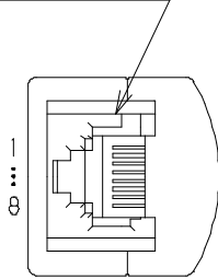
MJ1 (8極8心RJ48)
