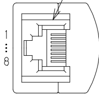
MJ1 (8極8心RJ45)
