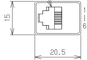
MJ2 (6極 6心)
